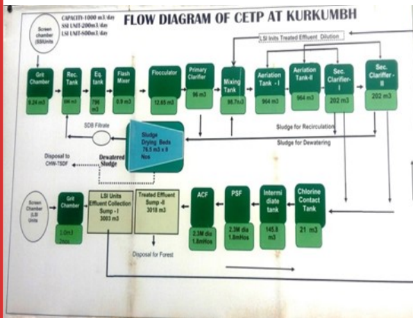
Flow diagram of CETP
